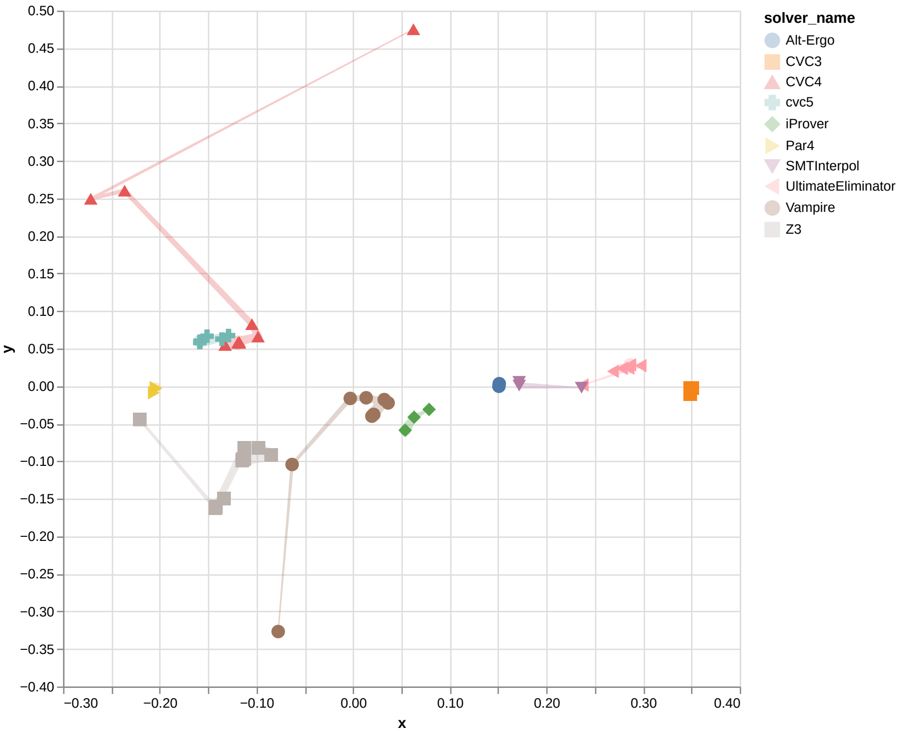
Isomap with cosine for UFNIA
