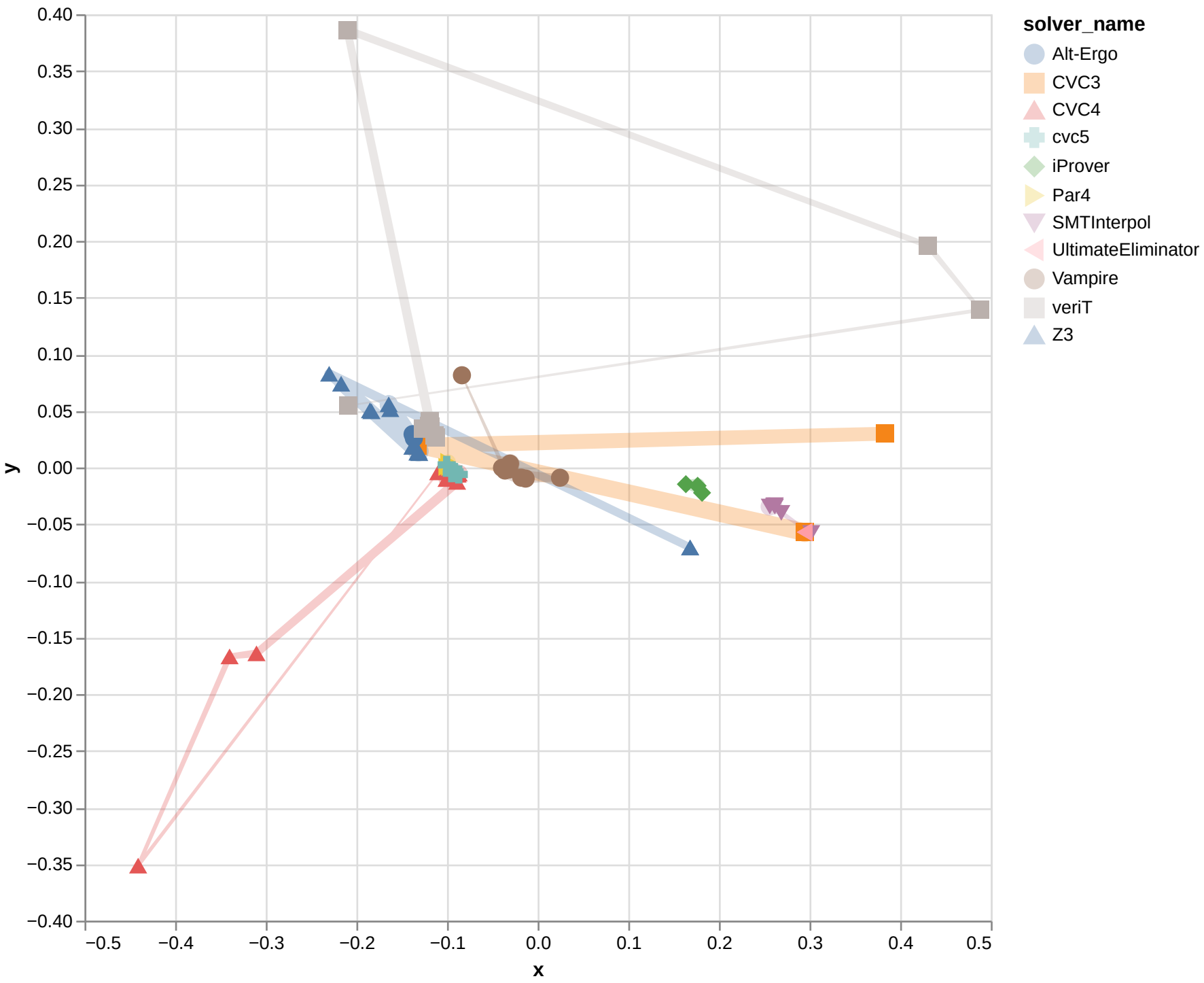
Isomap with cosine for UFLIA
