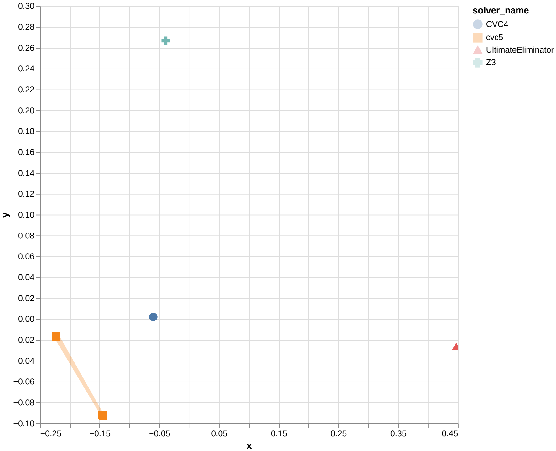
Isomap with cosine for UFFPDTNIRA
