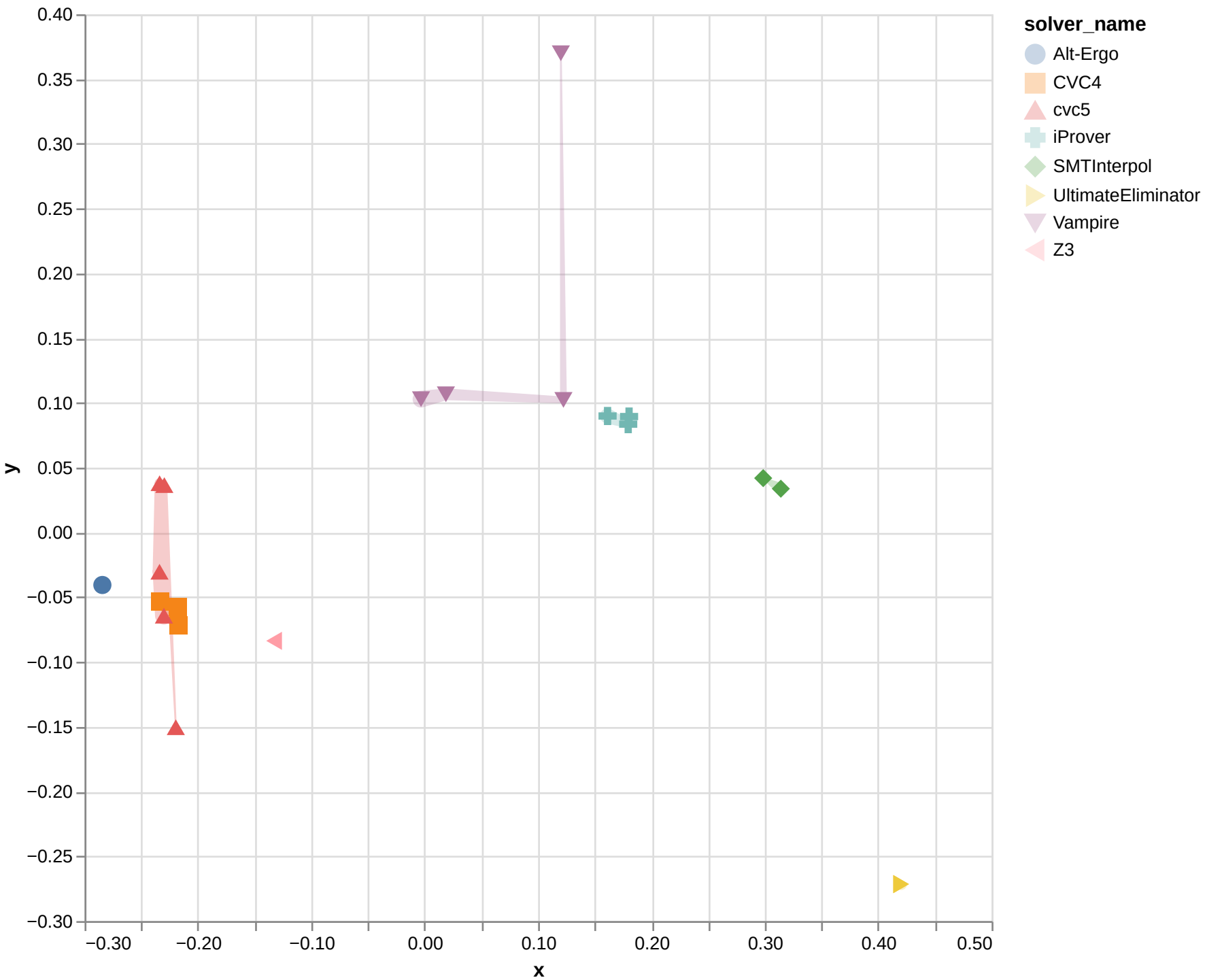
Isomap with cosine for UFDTNIRA
