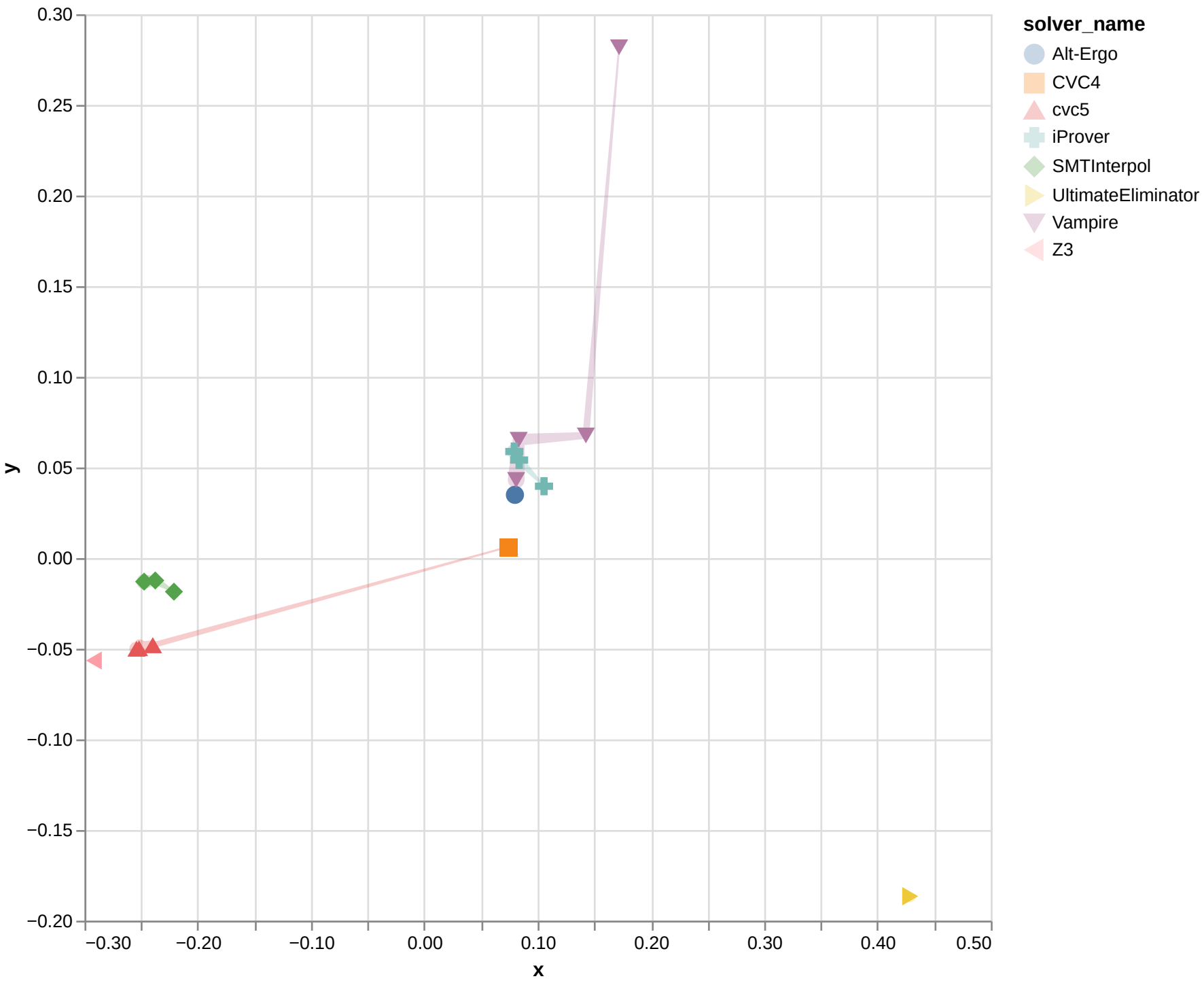
Isomap with cosine for UFDTLIRA
