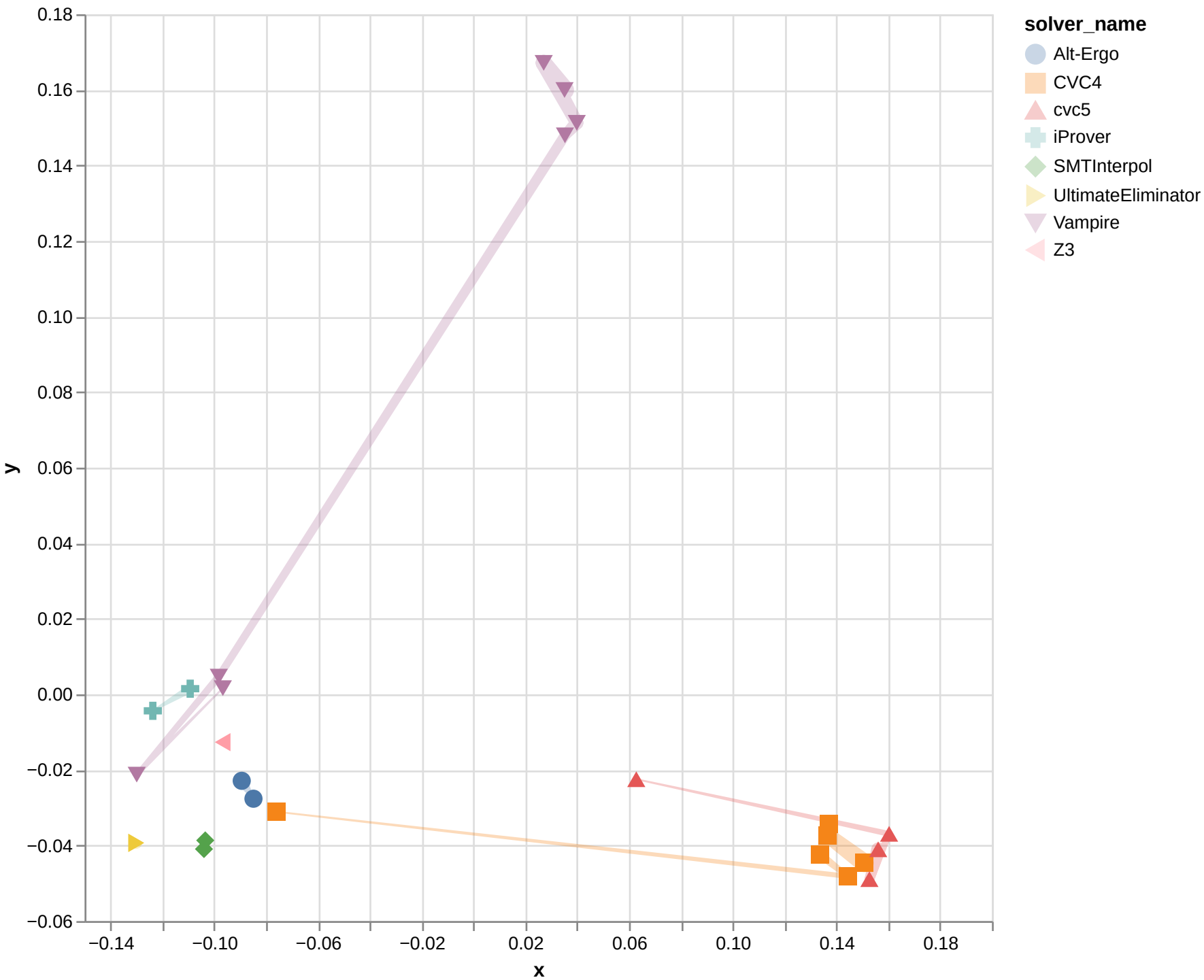
Isomap with cosine for UFDTLIA
