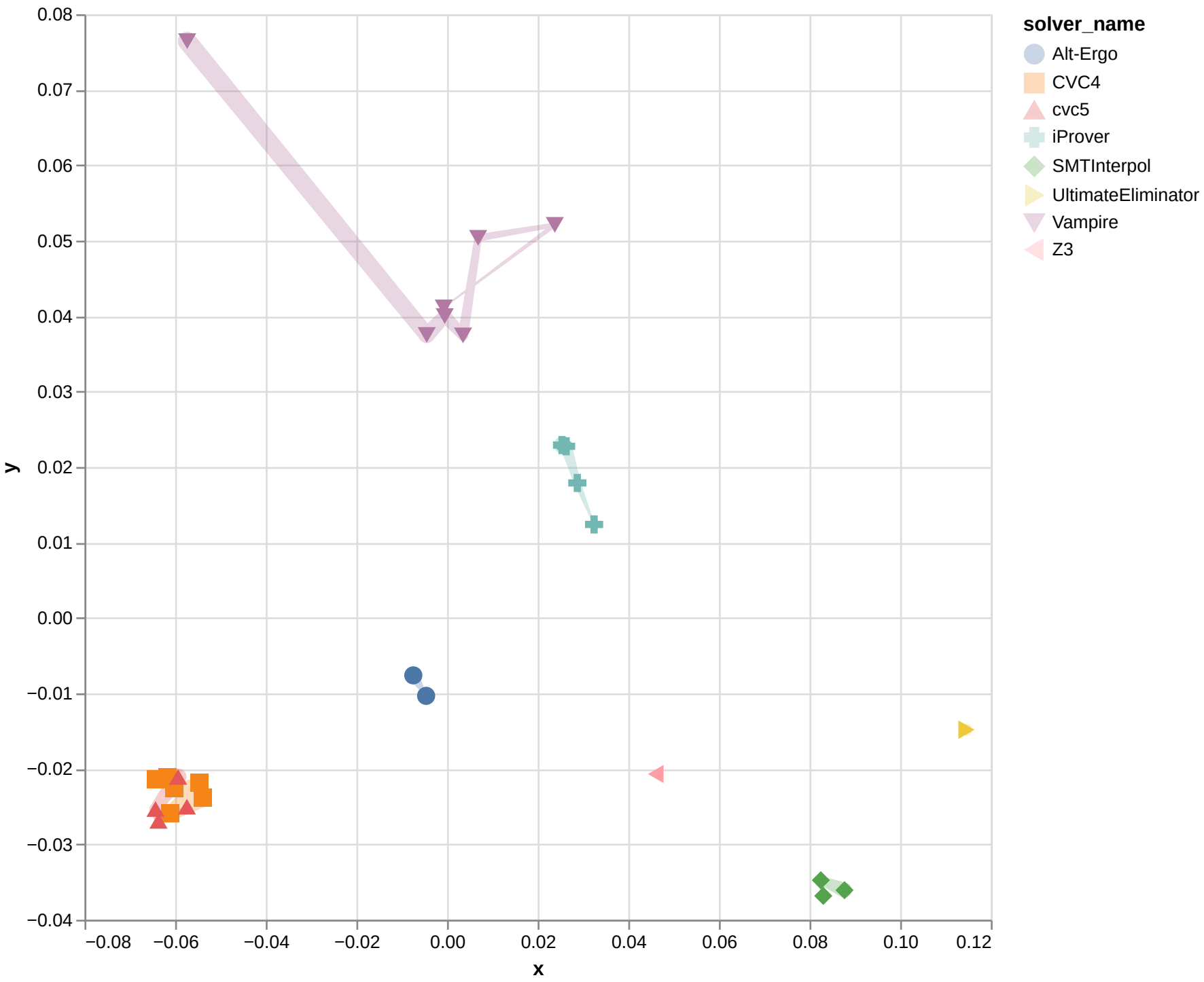
Isomap with cosine for UFDT
