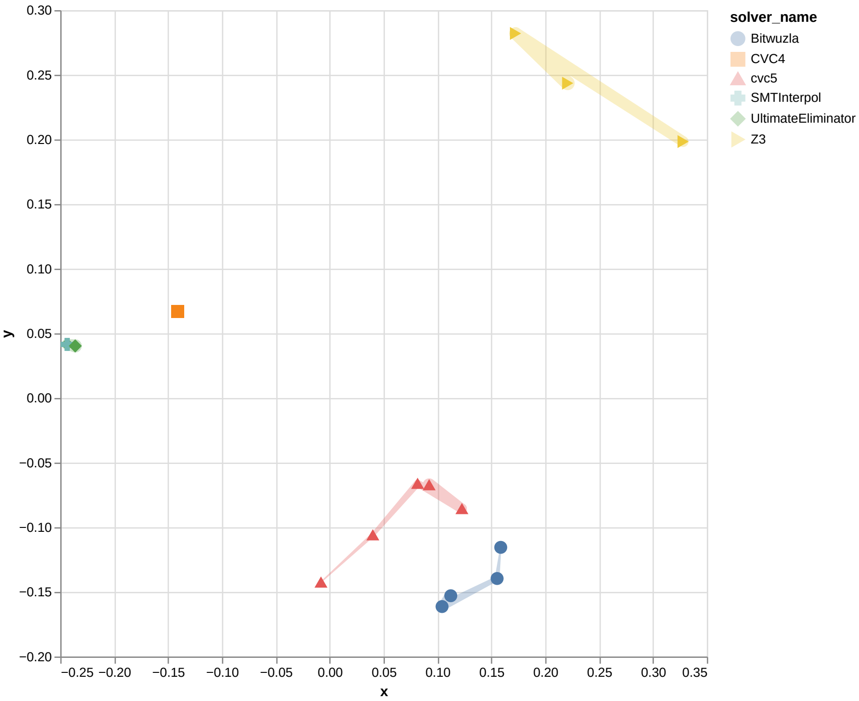
Isomap with cosine for UFBV
