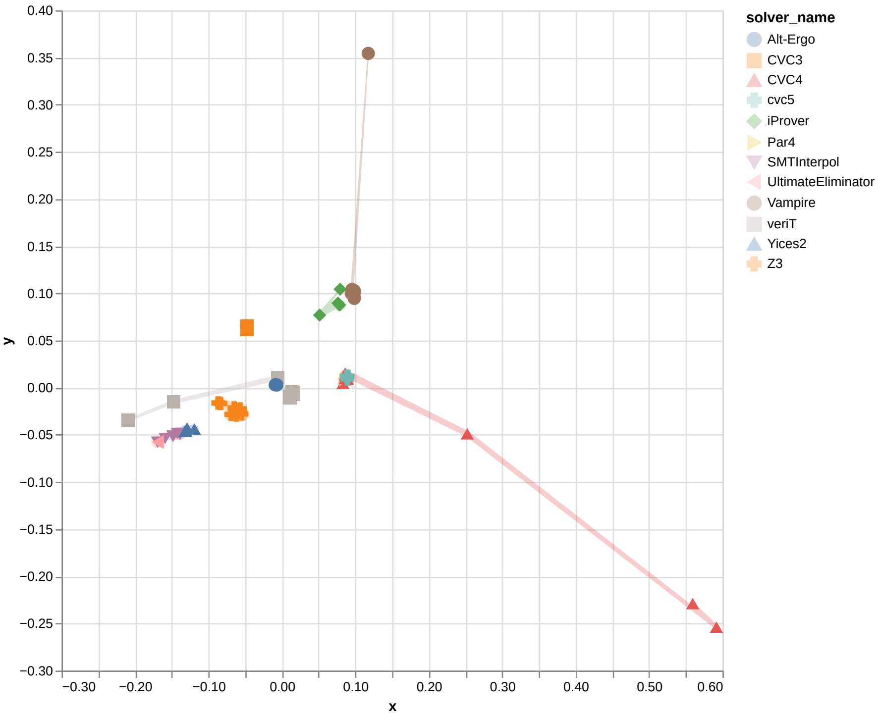
Isomap with cosine for UF
