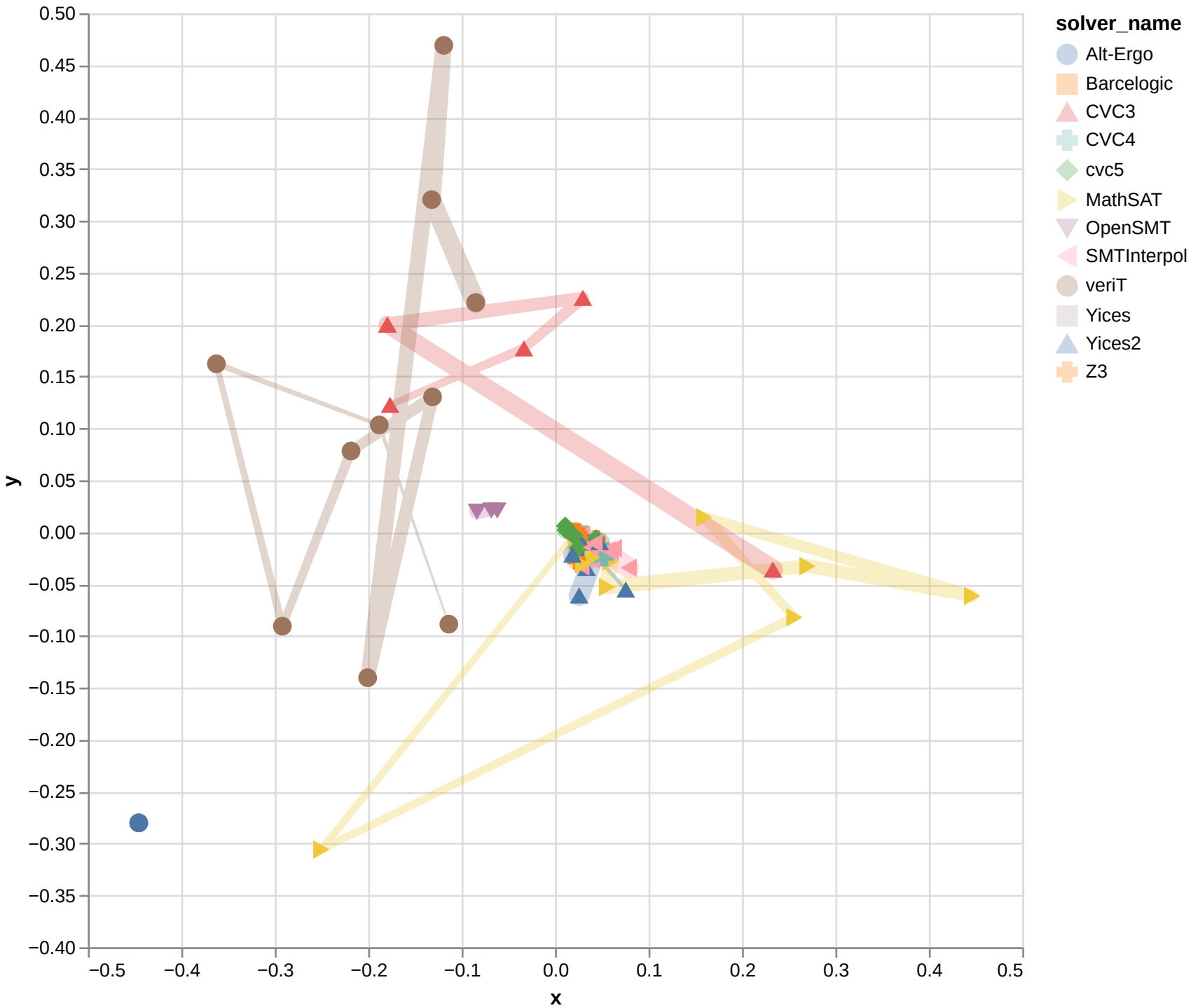
Isomap with cosine for QF_UFLIA
