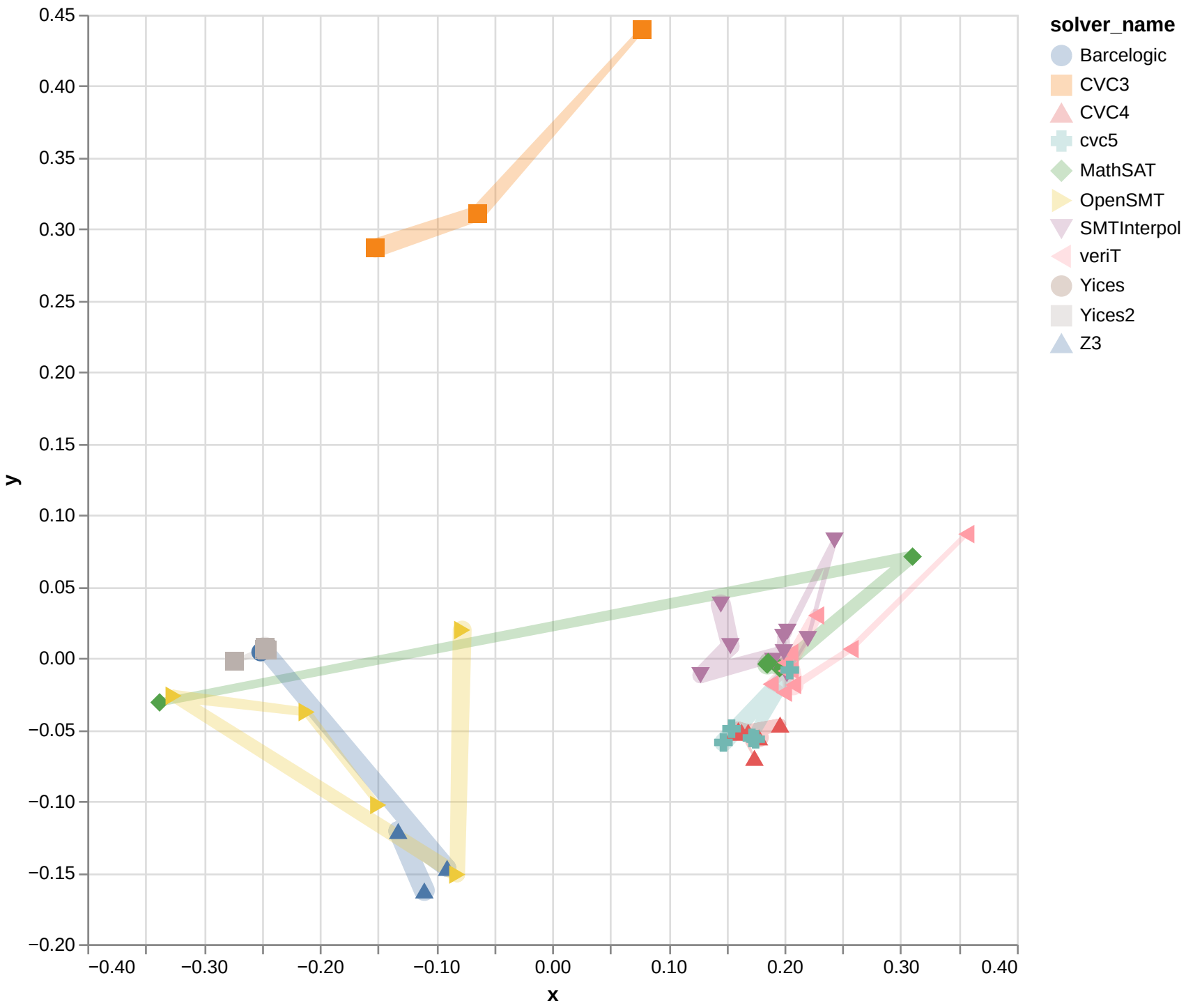
Isomap with cosine for QF_UFIDL
