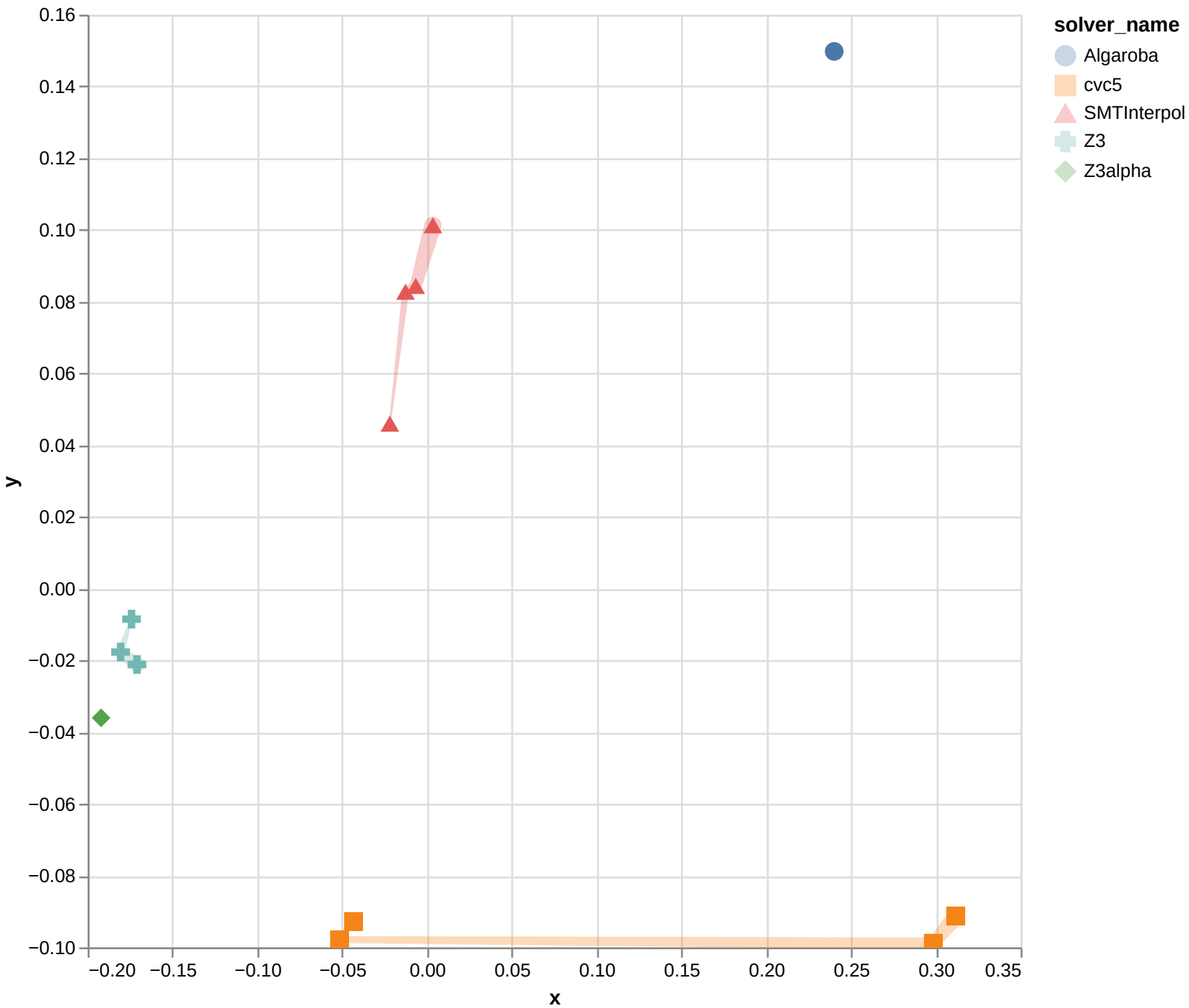
Isomap with cosine for QF_UFDT
