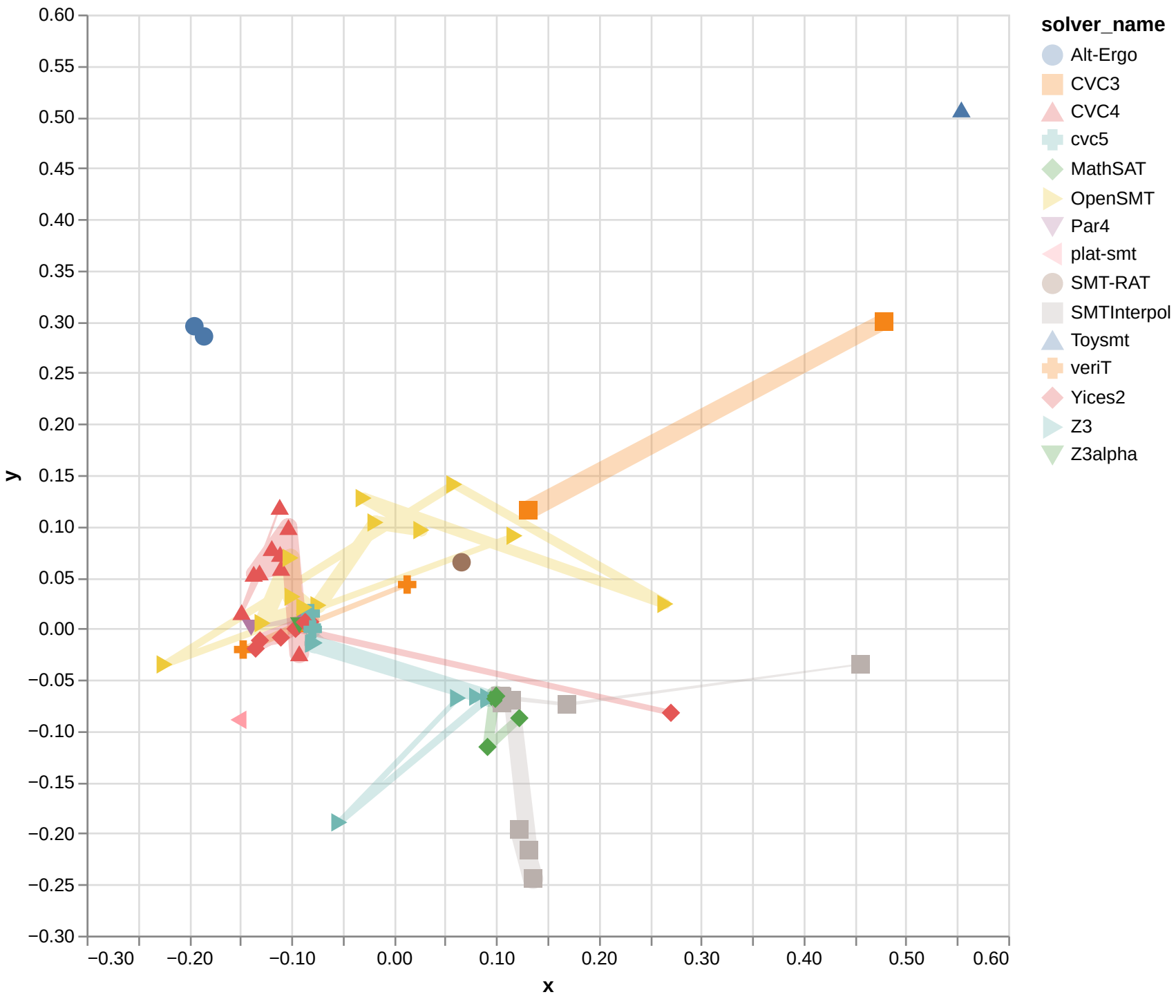
Isomap with cosine for QF_UF
