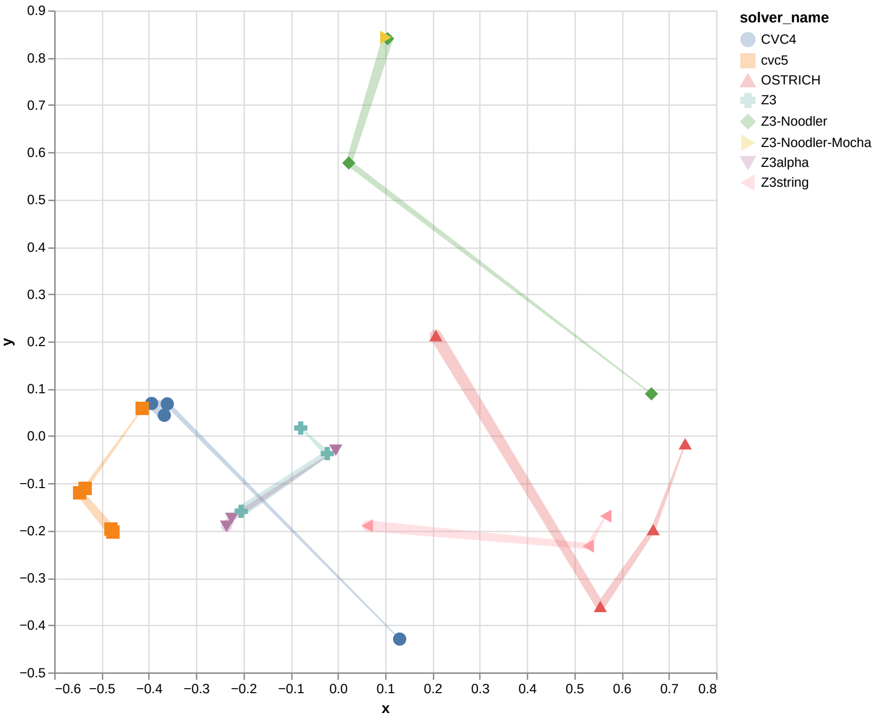
Isomap with cosine for QF_SLIA
