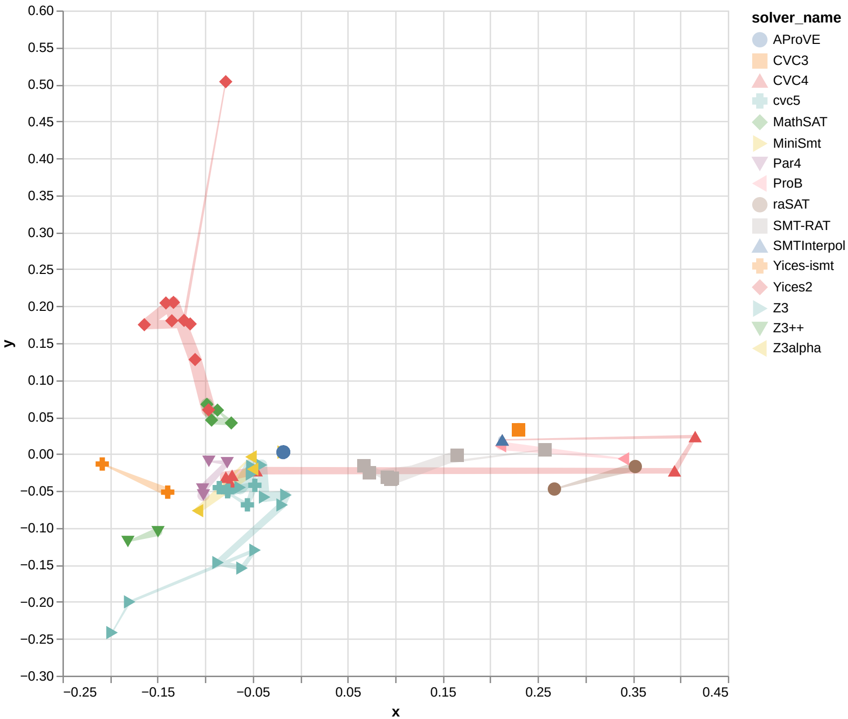
Isomap with cosine for QF_NIA
