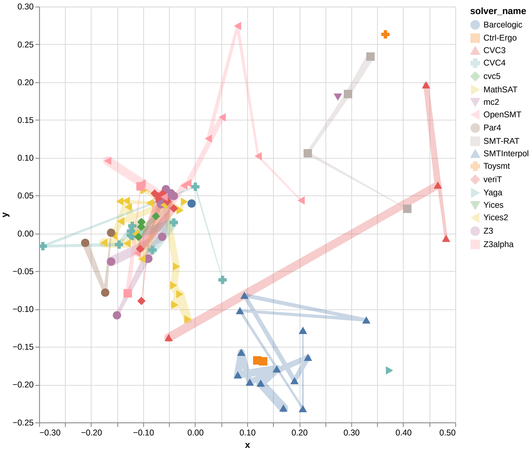
Isomap with cosine for QF_LRA
