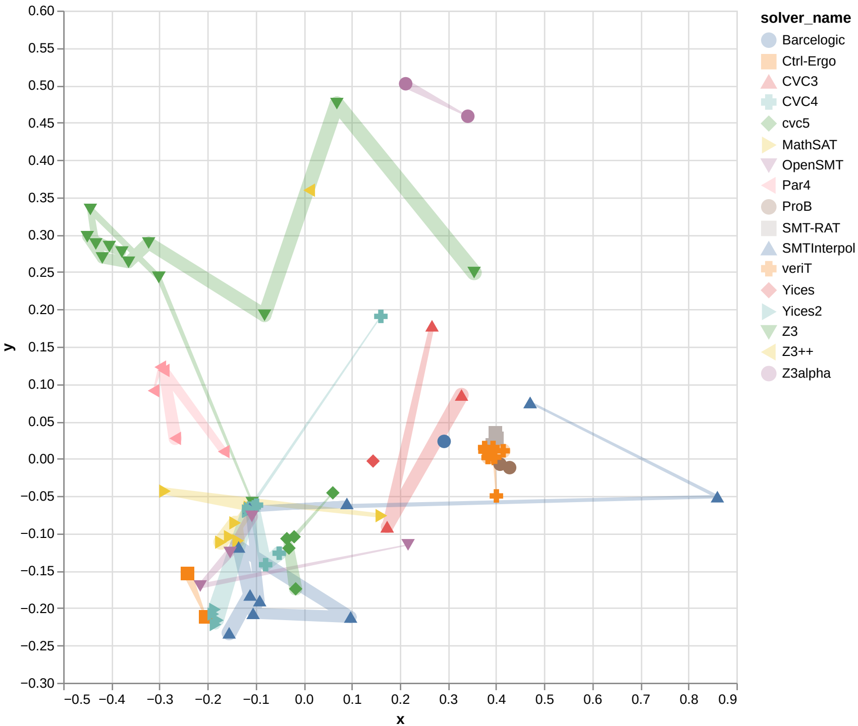
Isomap with cosine for QF_LIA
