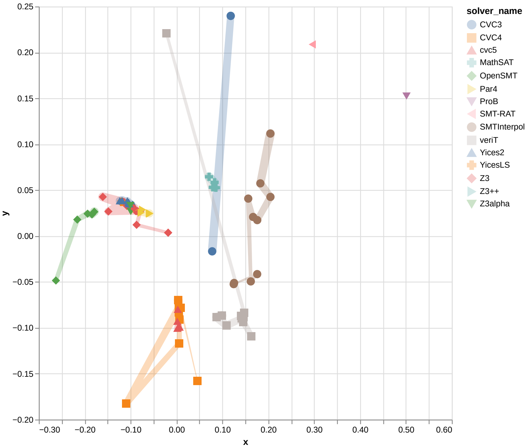
Isomap with cosine for QF_IDL
