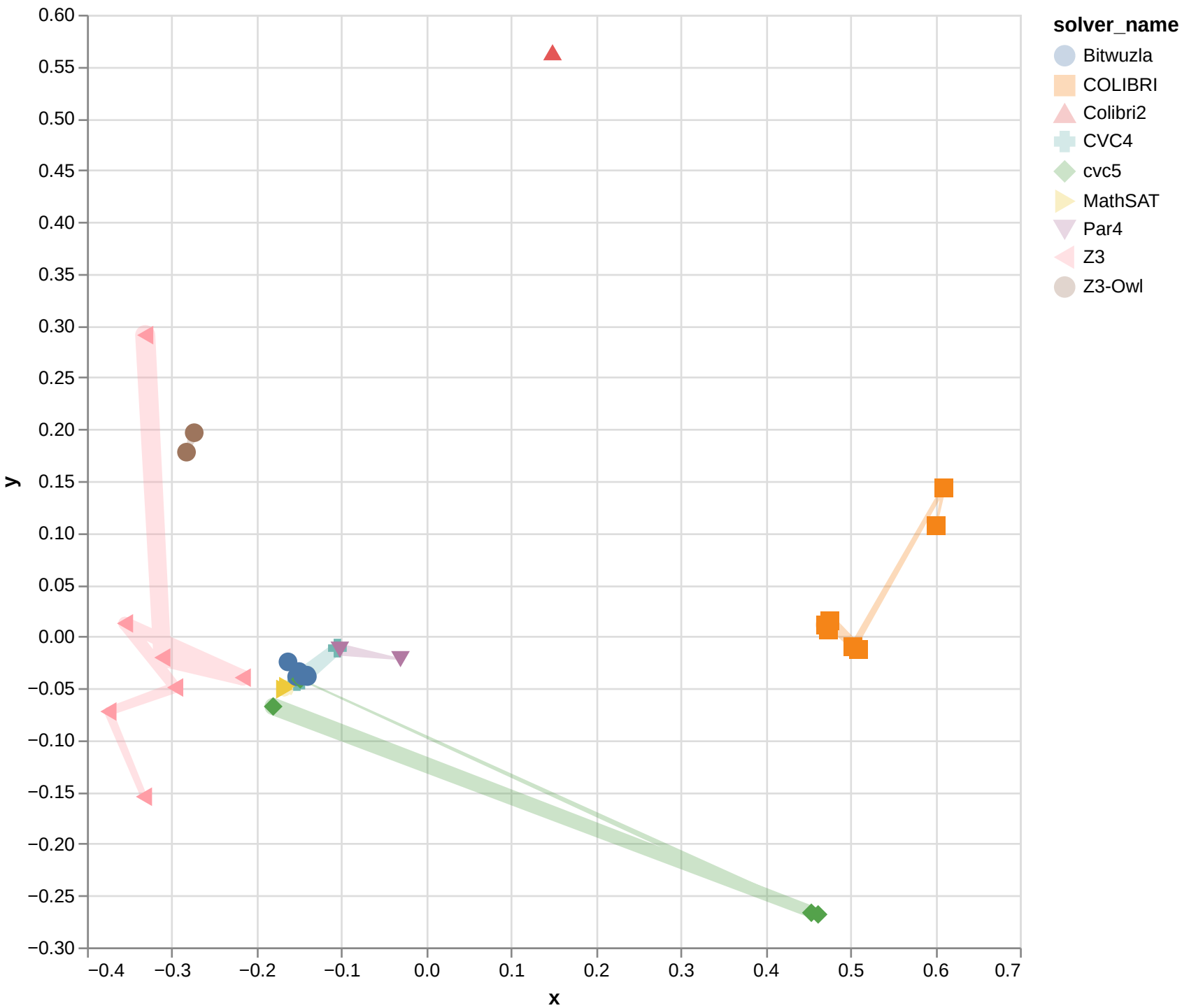
Isomap with cosine for QF_BVFP
