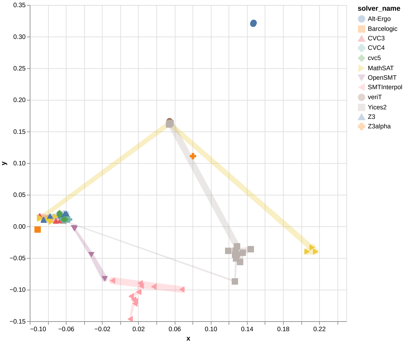
Isomap with cosine for QF_AX
