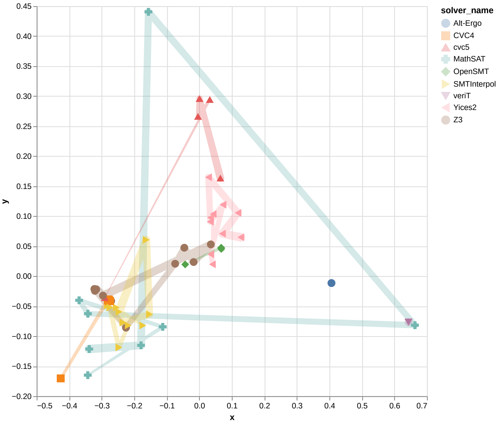
Isomap with cosine for QF_ALIA
