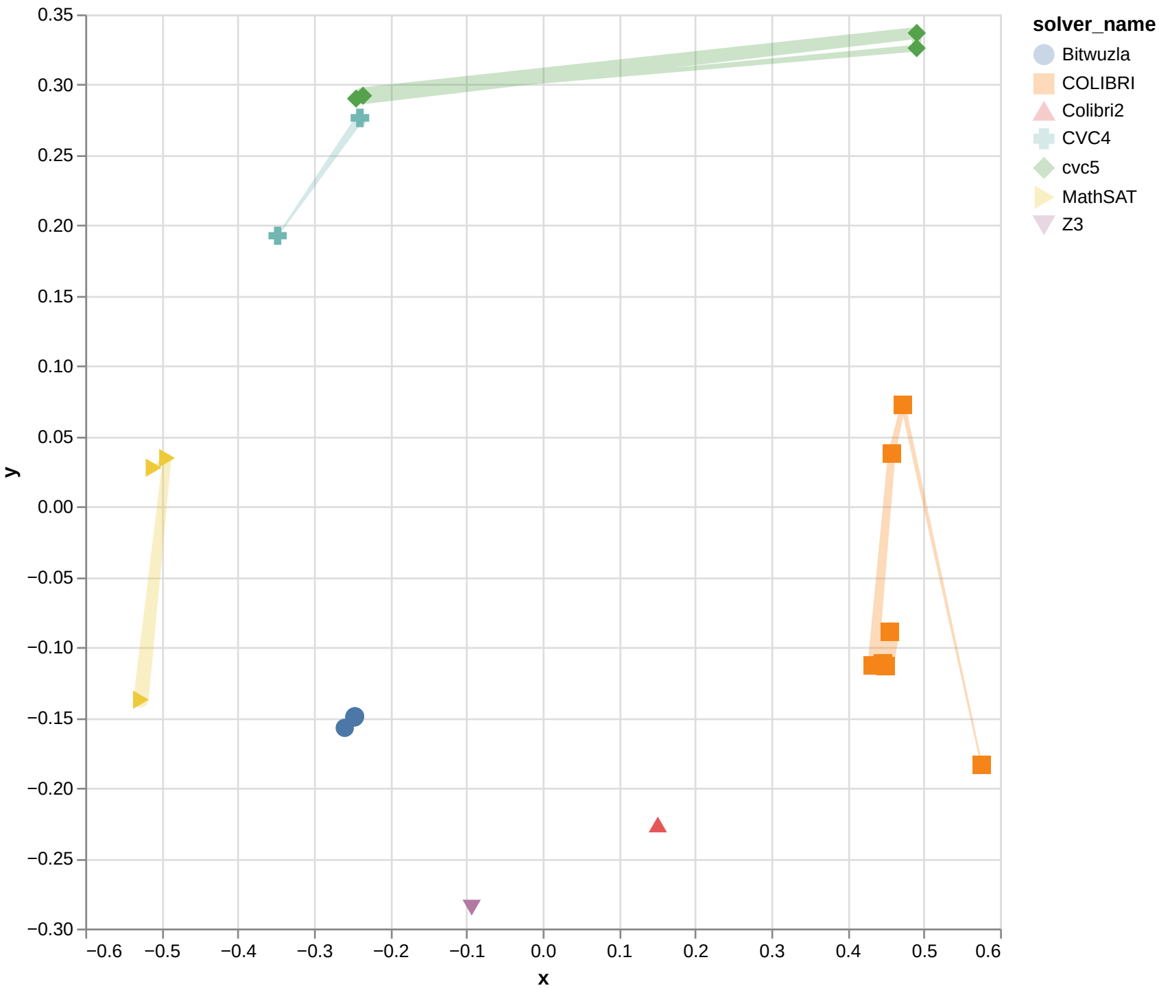
Isomap with cosine for QF_ABVFP
