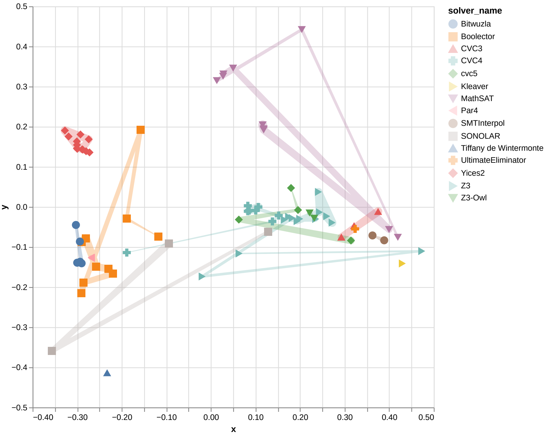
Isomap with cosine for QF_ABV
