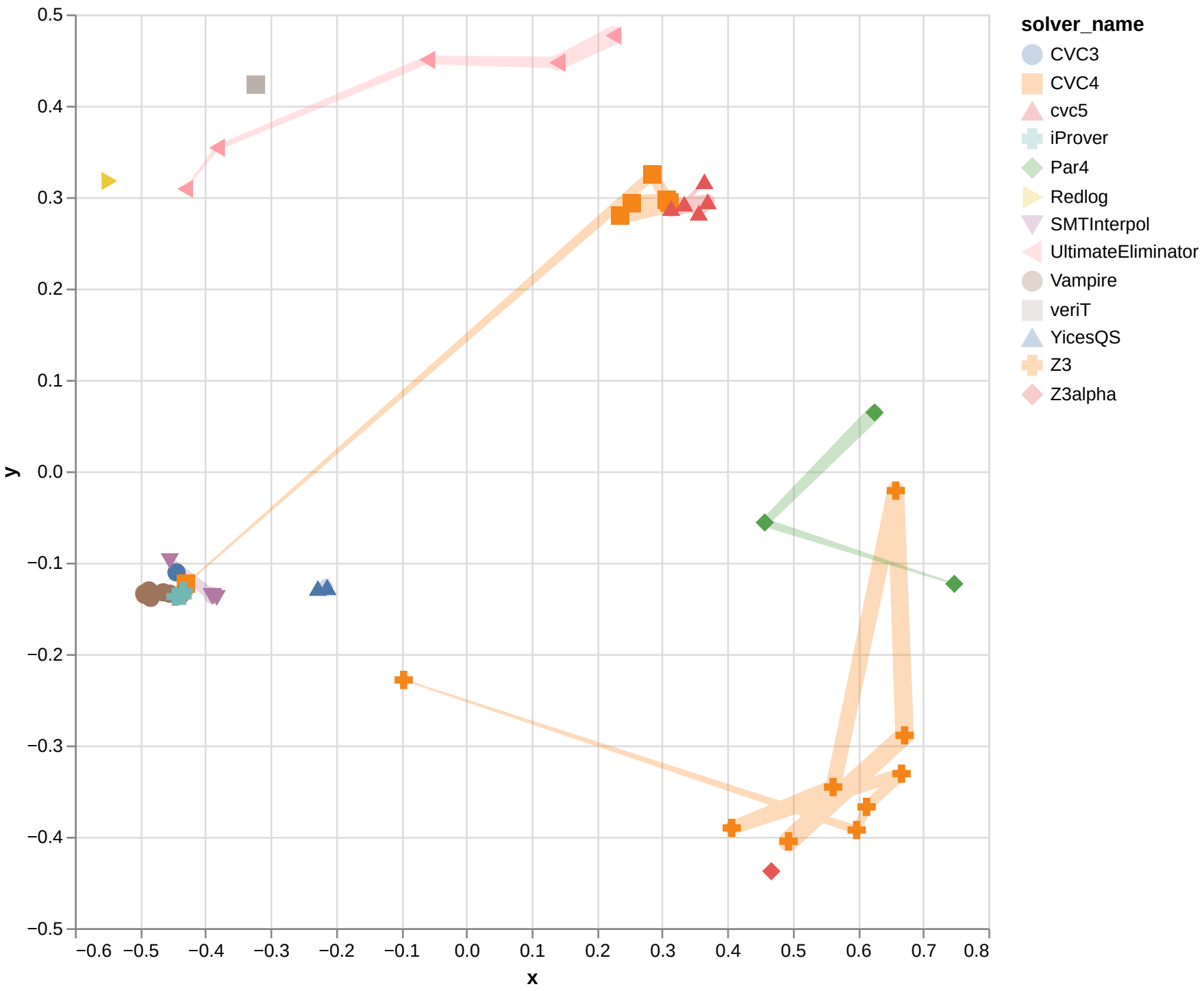
Isomap with cosine for LRA
