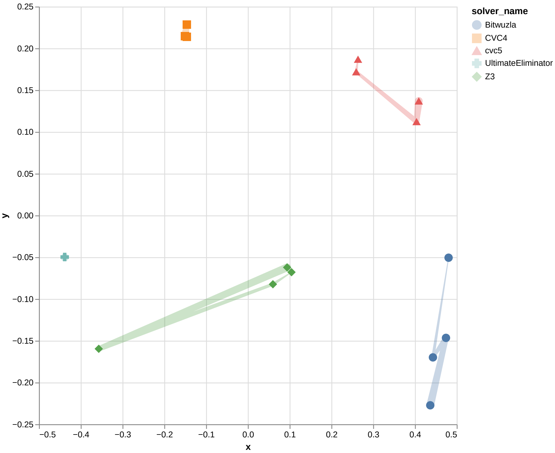
Isomap with cosine for FP
