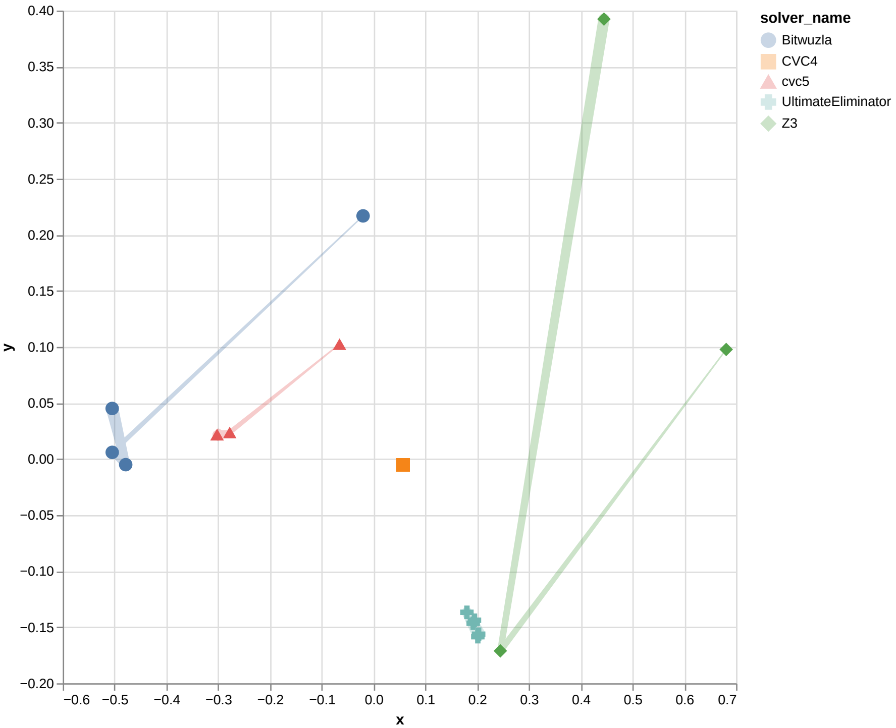
Isomap with cosine for BVFP
