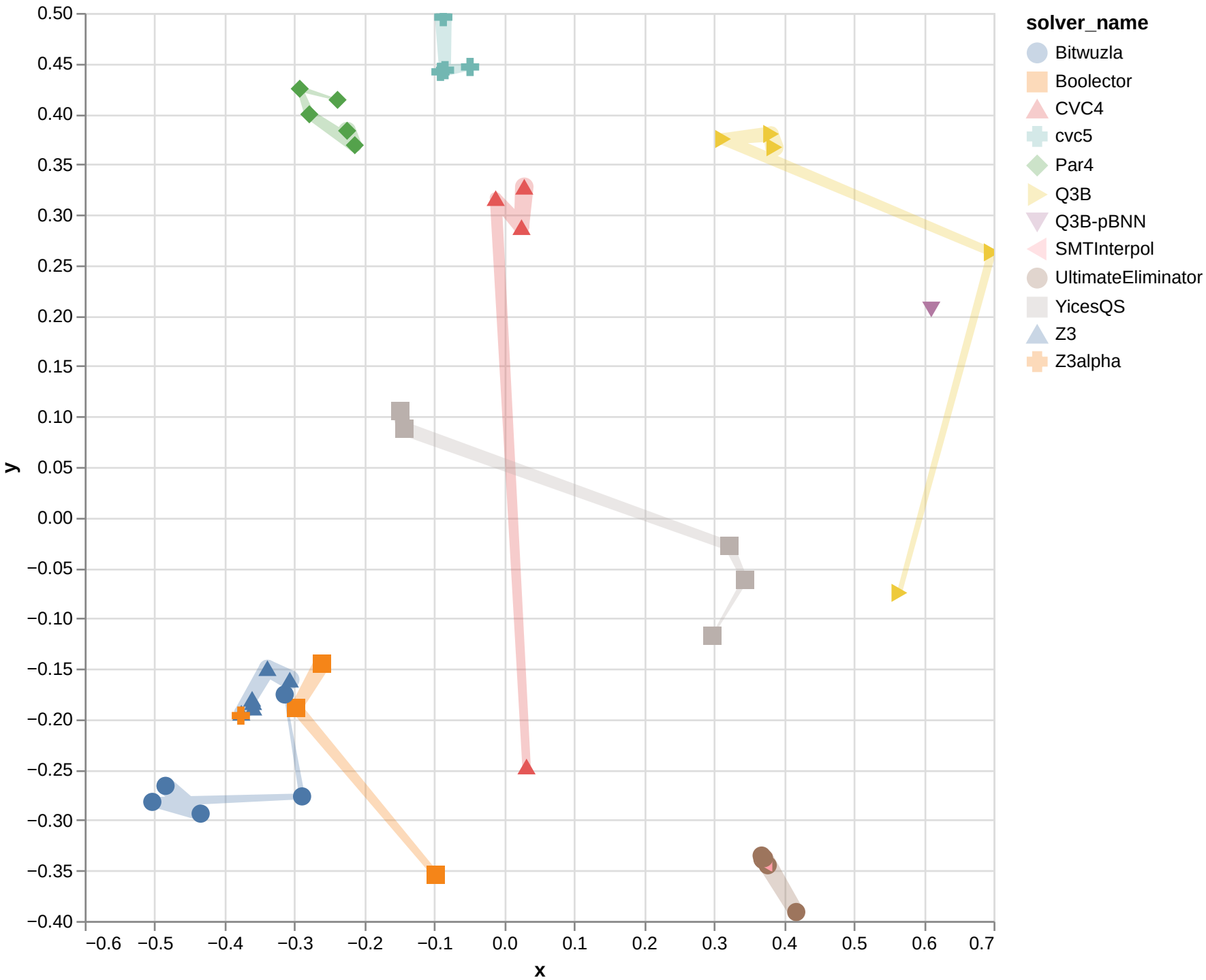
Isomap with cosine for BV
